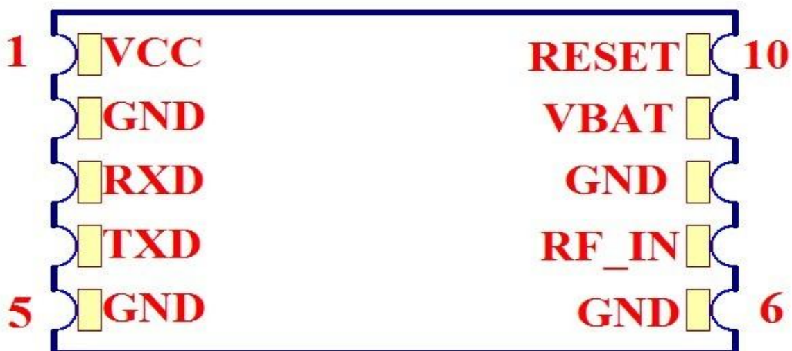
Figure 2: GT-1108-MTR Pin Package
