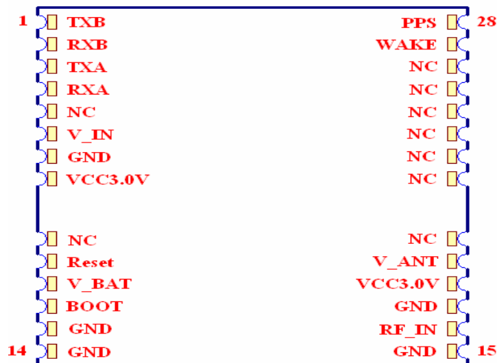
Figure 2: GT-2217-SF Pin Package
