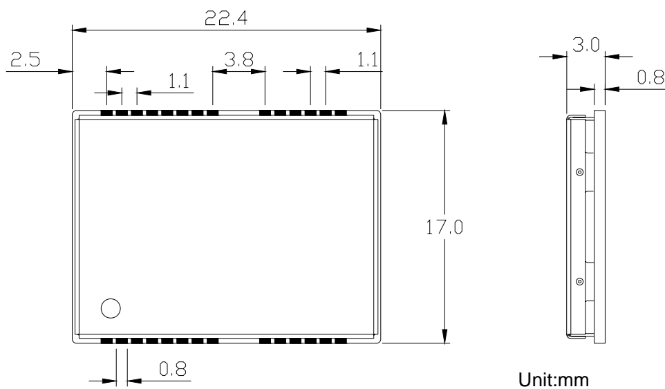
Figure 3: GT-2217-SF Dimensions
