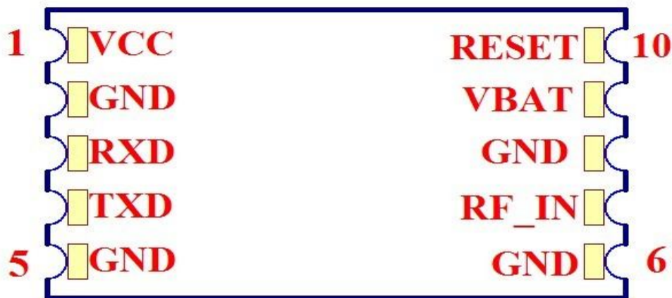
Figure 2: GT-1108-MT Pin Package
