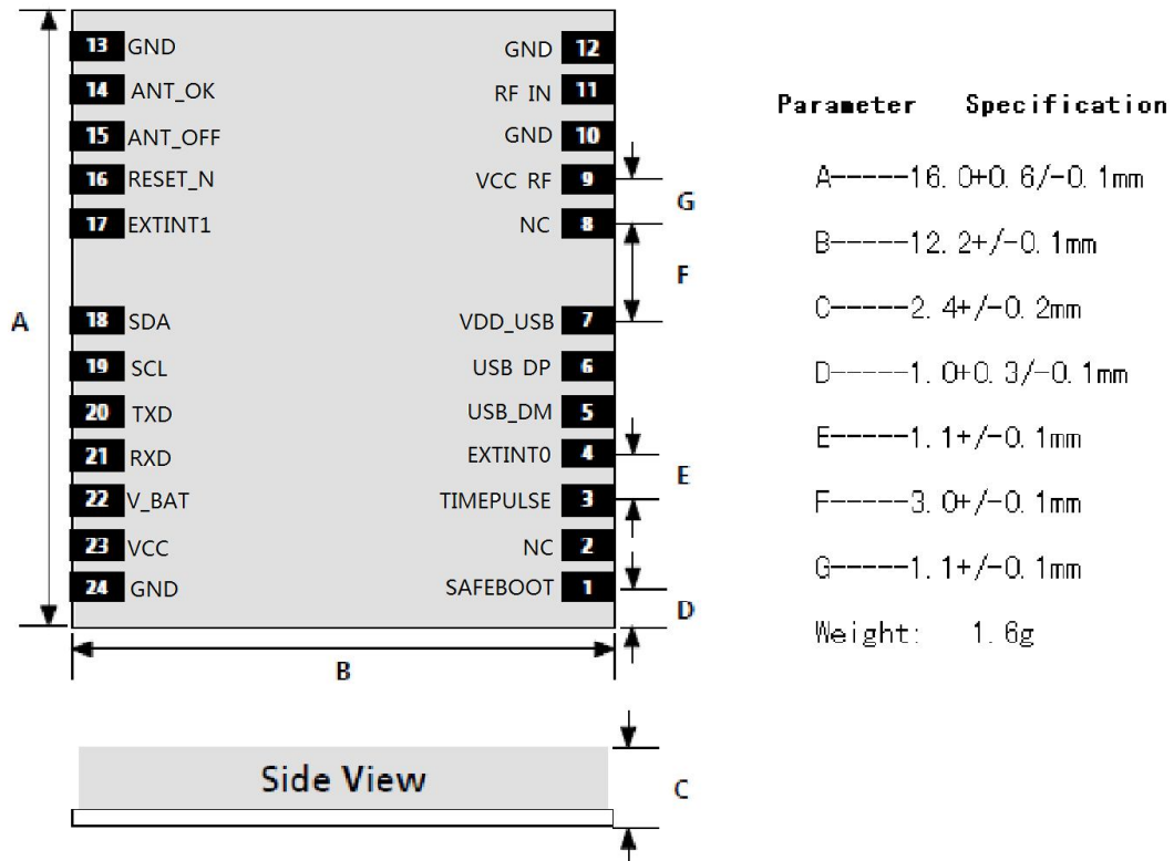
Figure 2: GT-1612-UB7X Pin Packag
